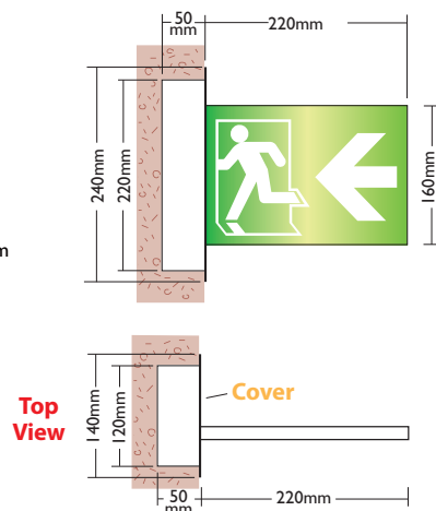
"CRYSTALITE" Cat. CX-LED-220-P-SOL-V-H Hairline s/s cover
