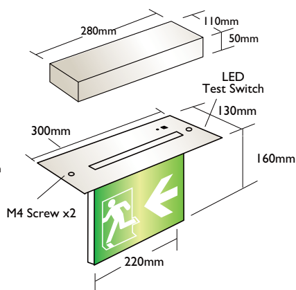
"CRYSTALITE" Cat. CX-LED-220-P-SOL
