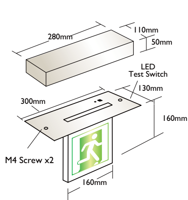
"CRYSTALITE" Cat. CX-LED-165-P-SOL
